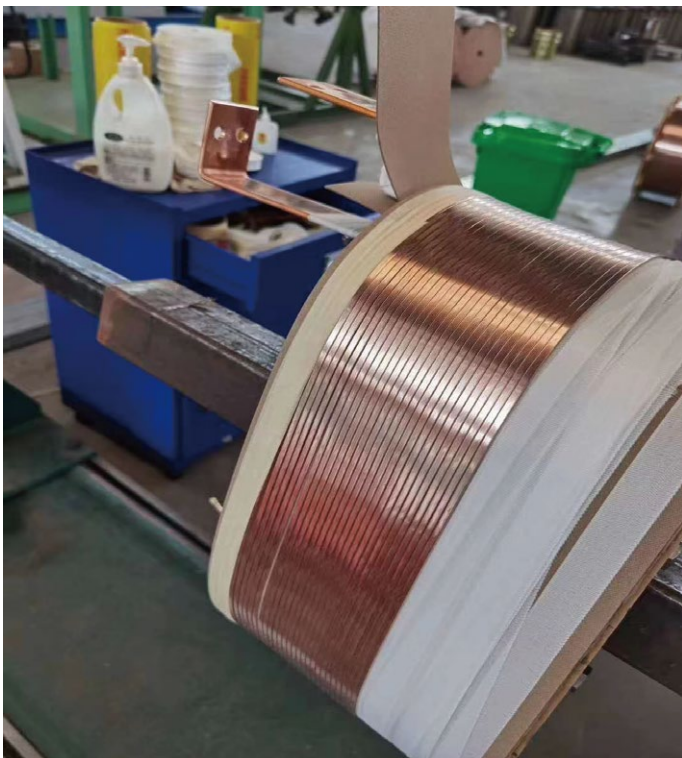
HV foil winding machine
